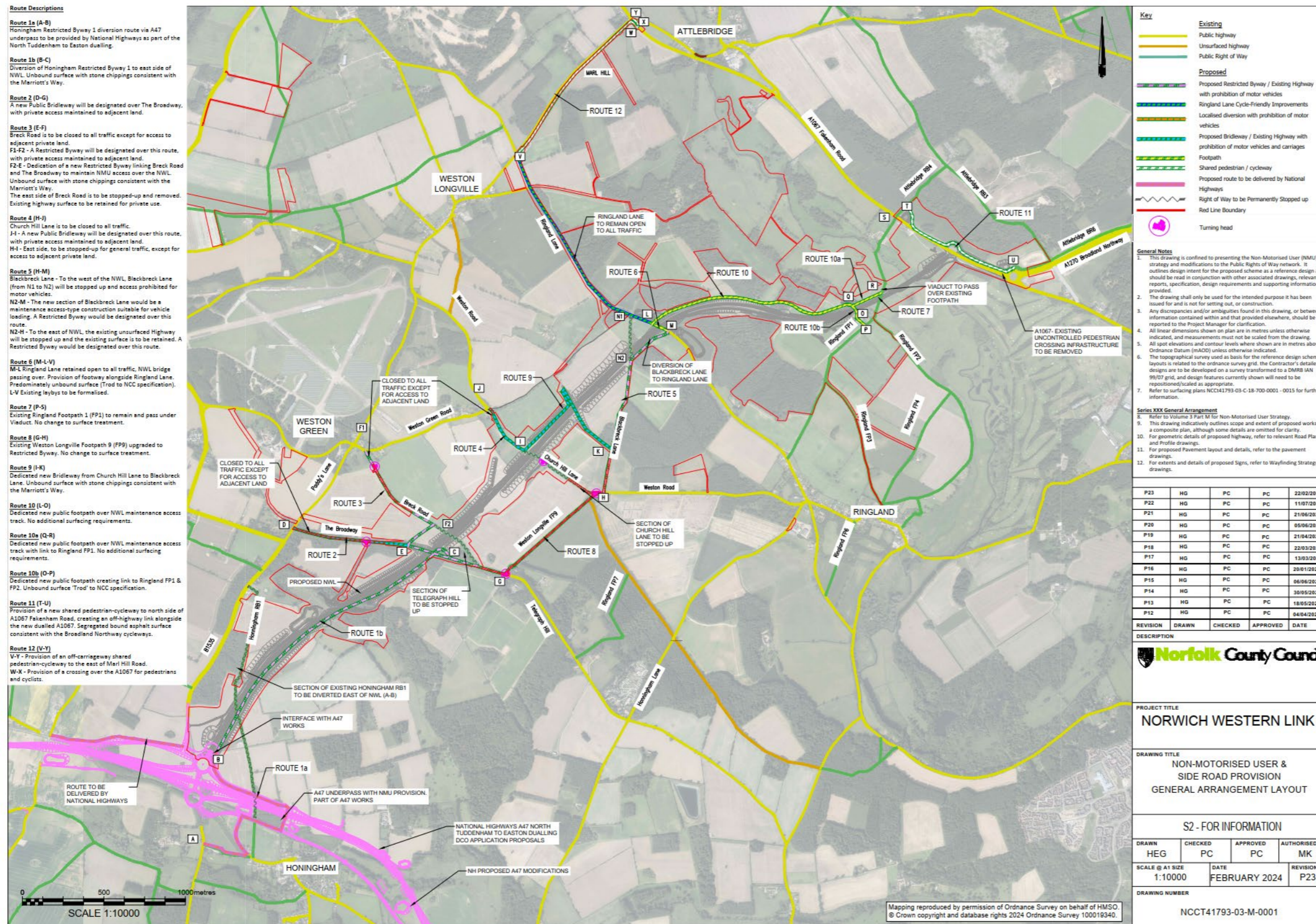
Figure 1-1 Location of new Public Rights of Way, and improvements to existing routes, to join up the active travel network
